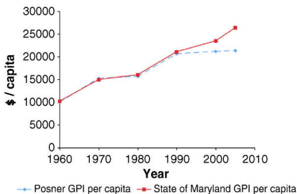
Fig. 2. Two estimates of the Maryland GPI derived independently.
