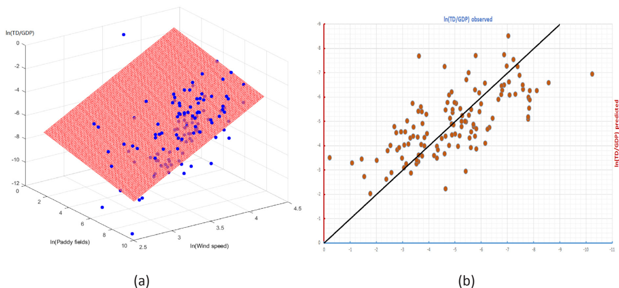
Fig. 3. Regression results: (a) The regression Model 2: \ln(\text{TD}/\text{GDP}) = -15.9936 + 3.6875 \cdot \ln(\text{wind speed at landfall}) - 0.2408 \cdot \ln(\text{area of paddy fields in typhoon swath}) , which is highlighted by red mesh and the observed 127 historical cases were scattered in blue points ( R^2 = 0.46 ); (b) \ln(\text{TD}/\text{GDP}) observed vs. predicted for Model 4 with fitness R^2 = 0.57 .
